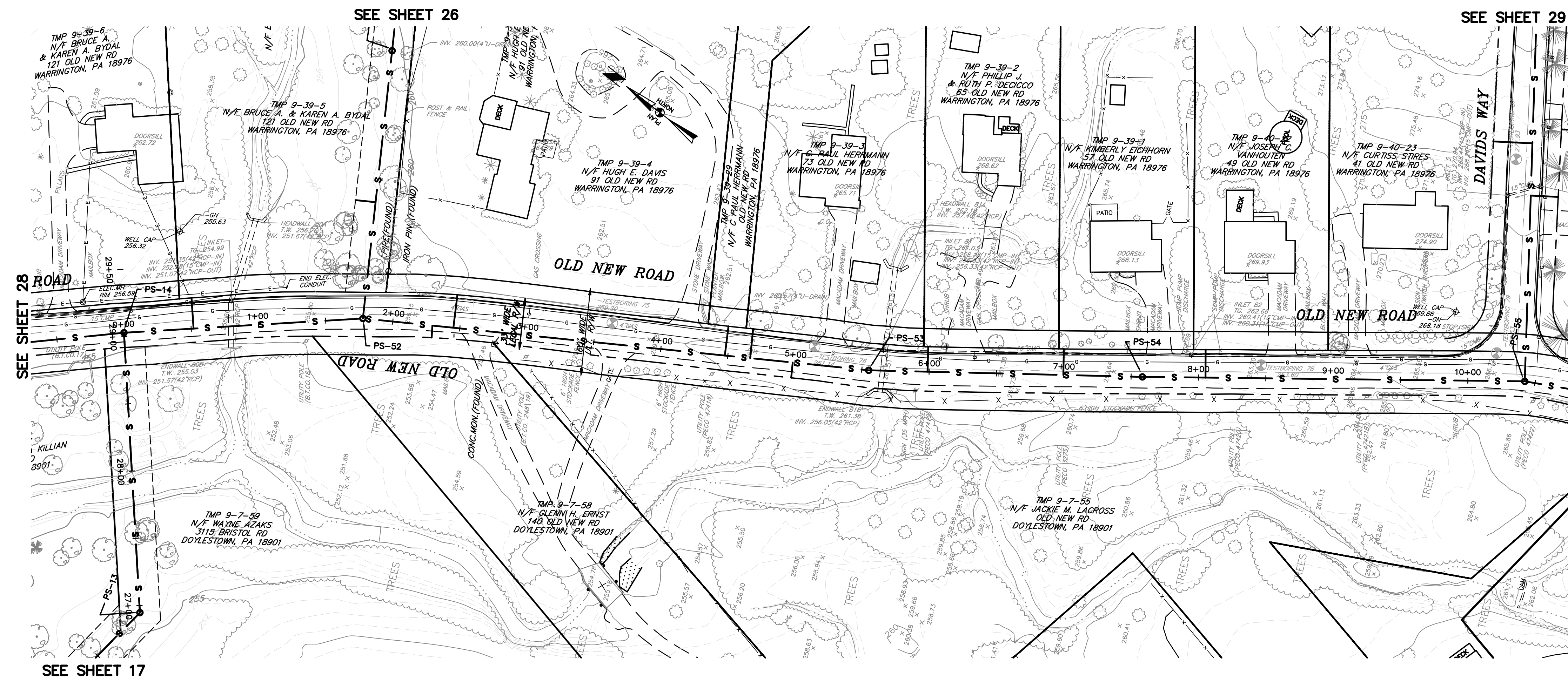
PLAN: OLD NEW ROAD
