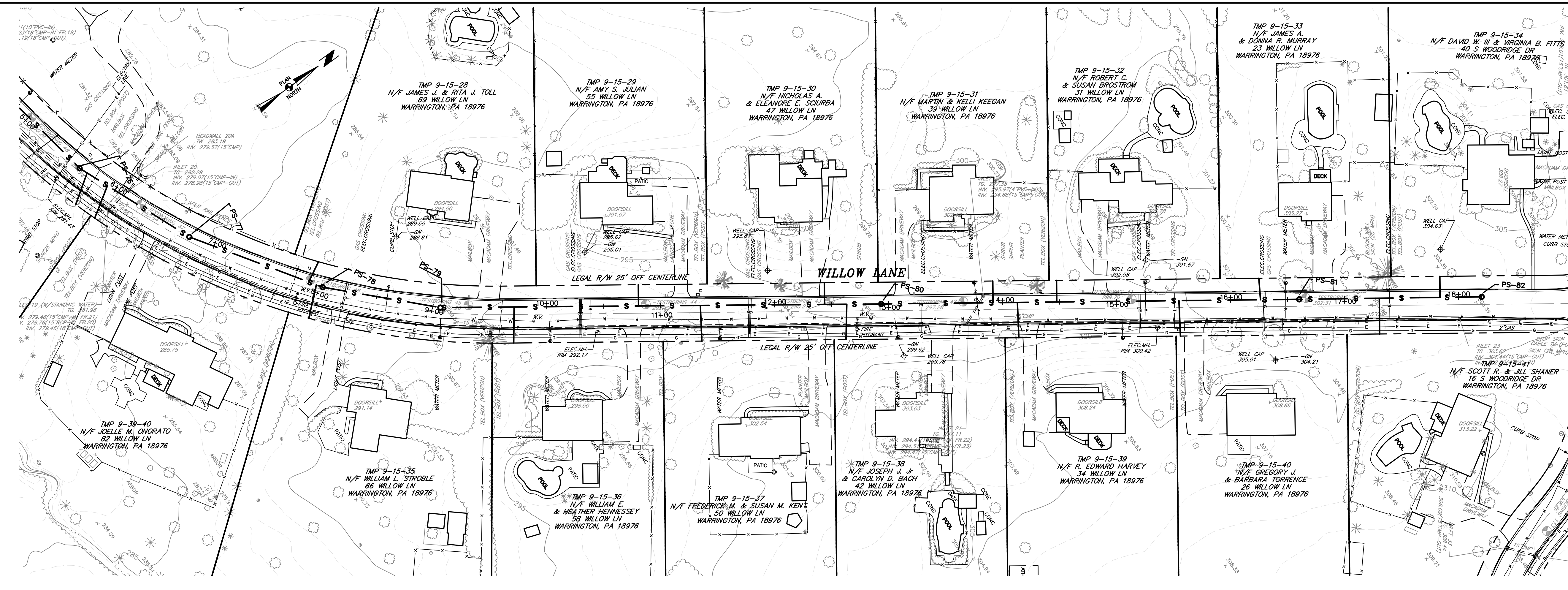
PLAN: WILLOW LANE SCALE: 1"=50'
