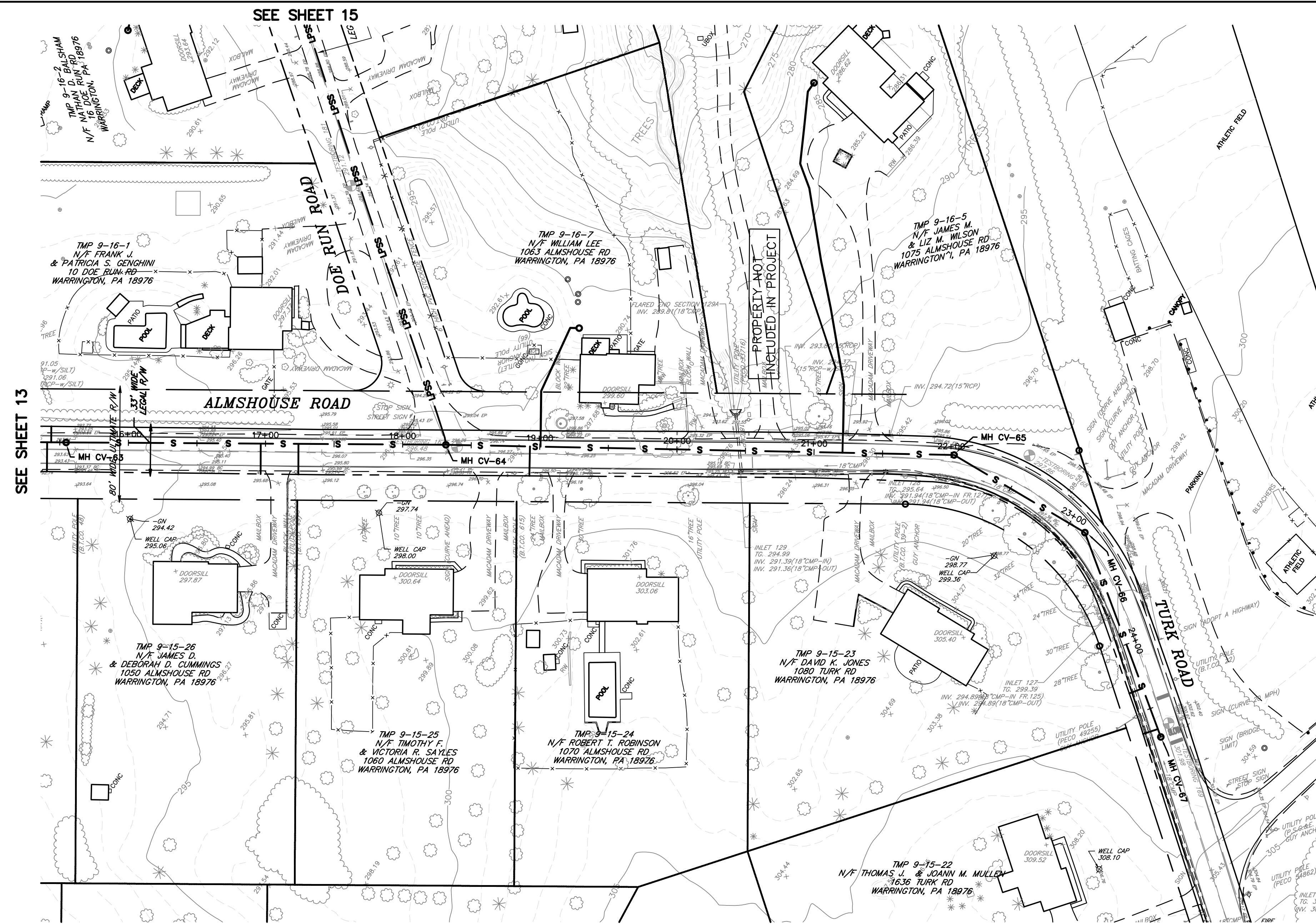
PLAN: ALMSHOUSE ROAD & TURK ROAD SCALE: 1"=50'
