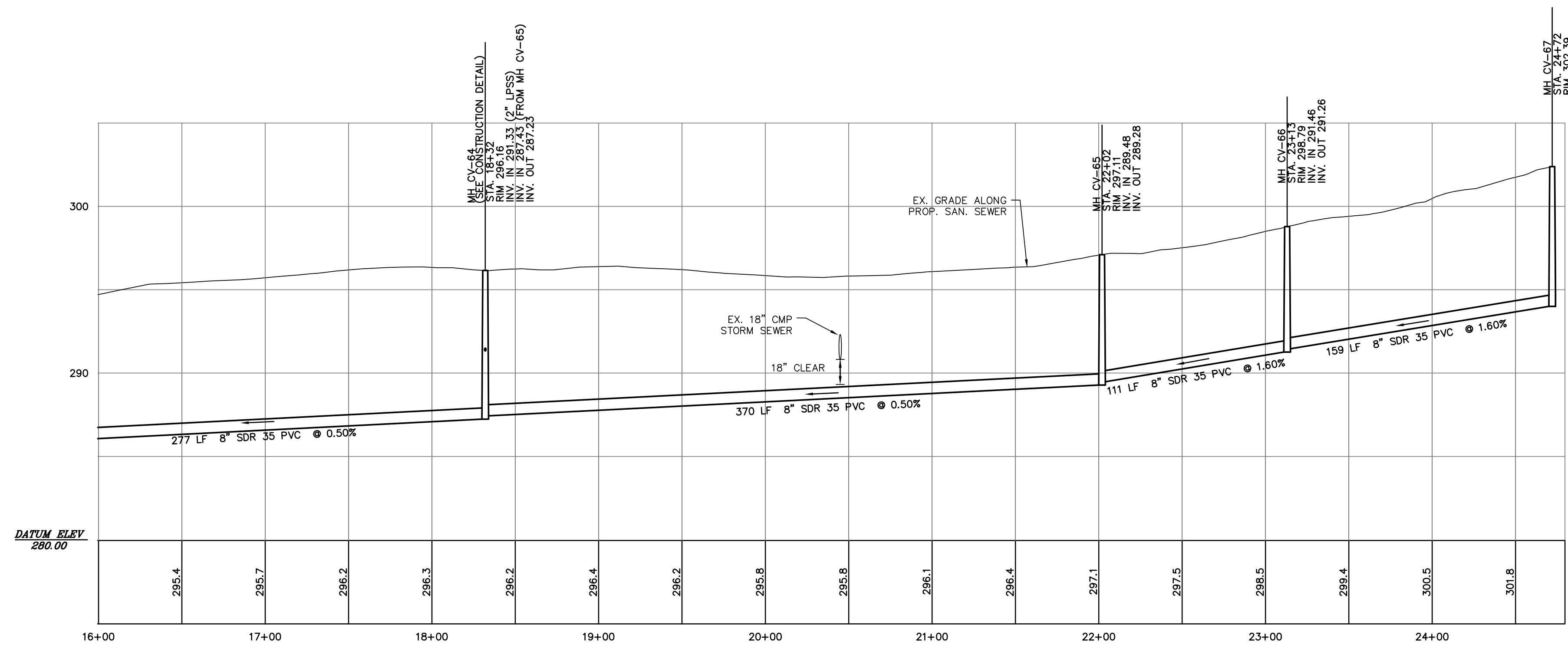
PROFILE: ALMSHOUSE ROAD & TURK ROAD (STA. 16+00 TO 24+72) SCALE: HORIZ. 1"=50' VERT. 1"=5'
