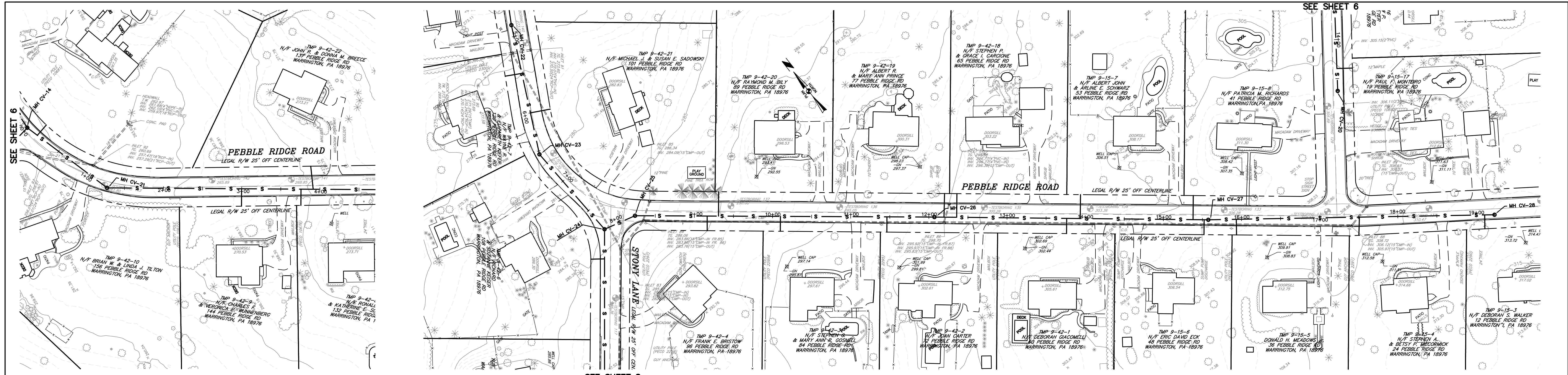
PLAN: PEBBLE RIDGE ROAD SCALE: 1"=50'
