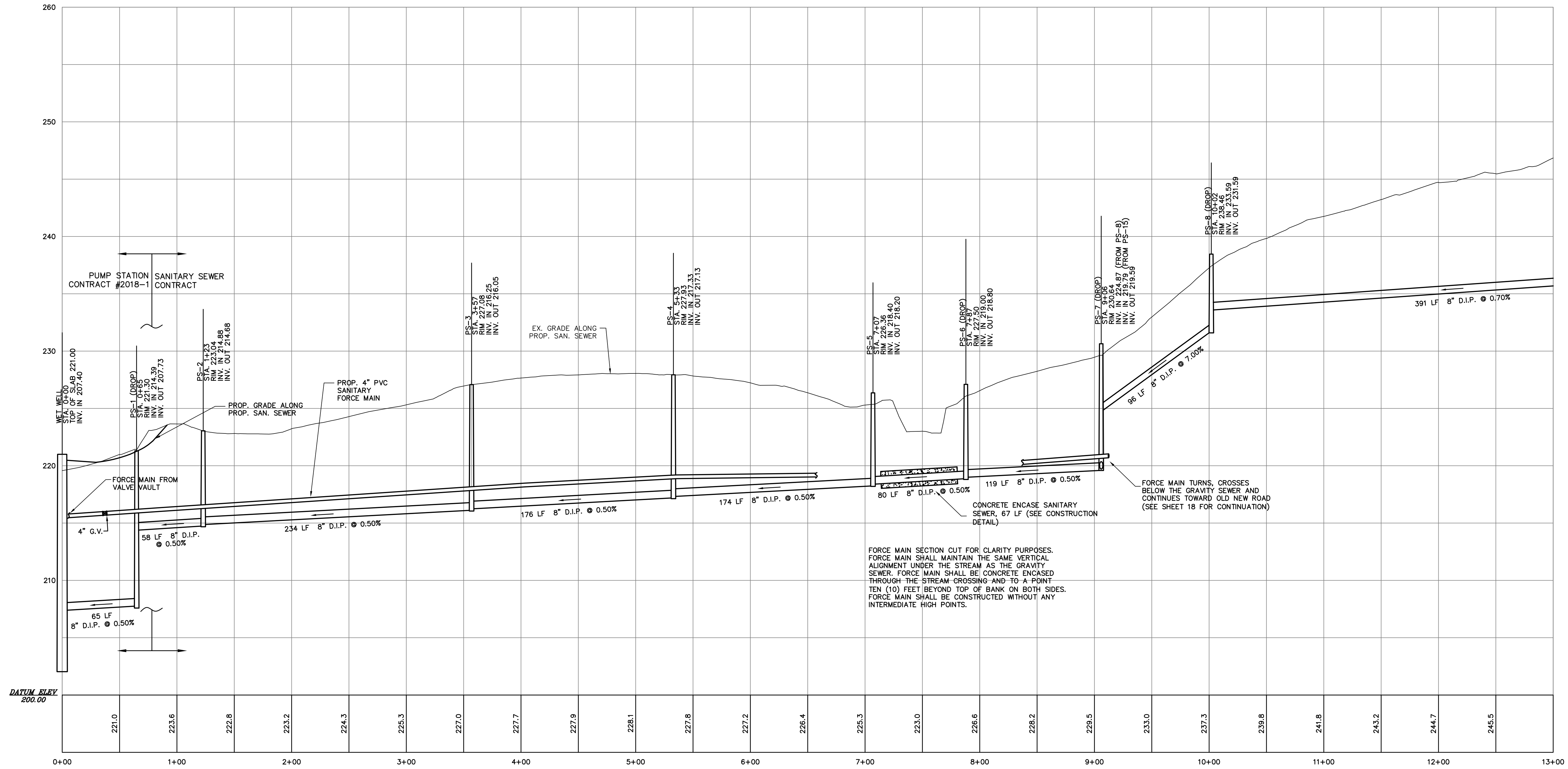
PROFILE: EASEMENTS TO PUMP STATION & OLD NEW ROAD, EAST RUN (STA. 0+00 TO 13+00) SCALE: HORIZ. 1"=50' VERT. 1"=5'
