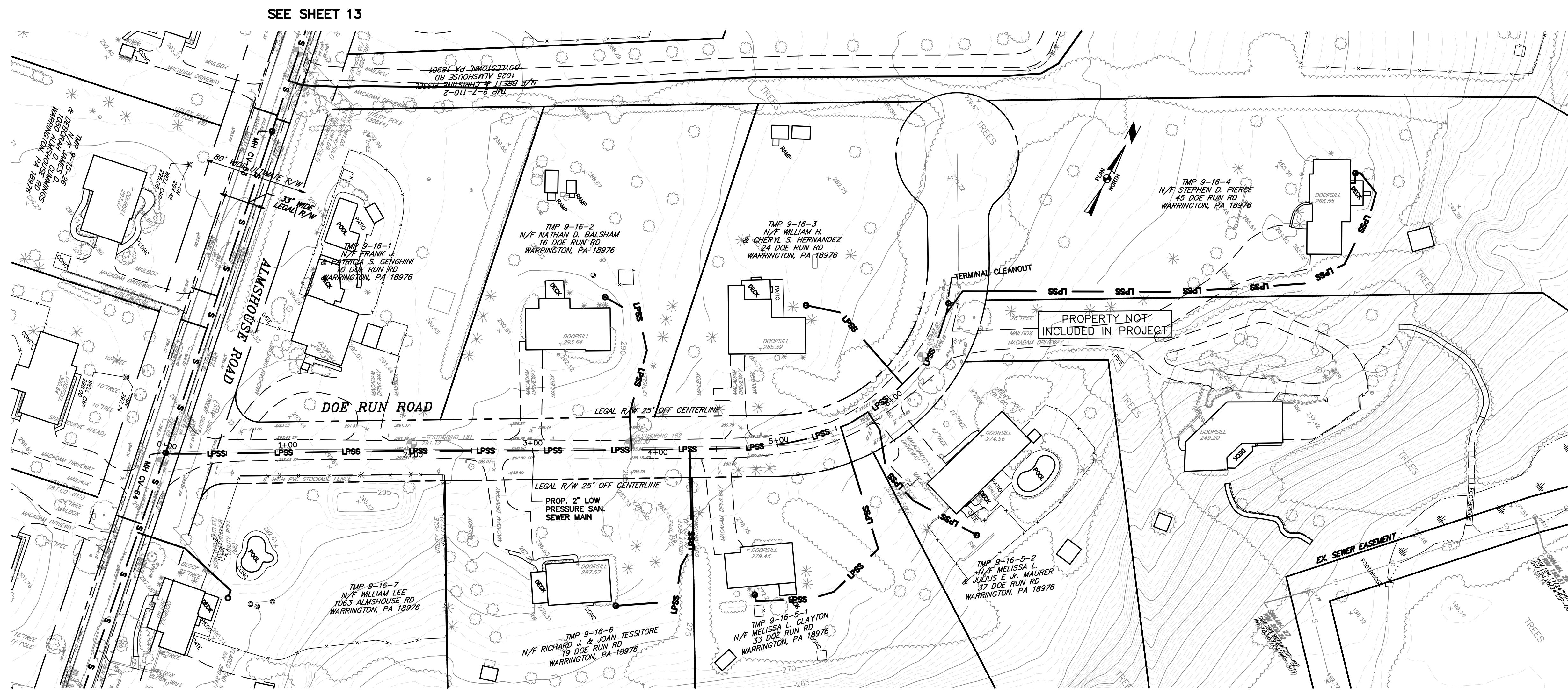
PLAN: DOE RUN ROAD SCALE: 1"=50'
