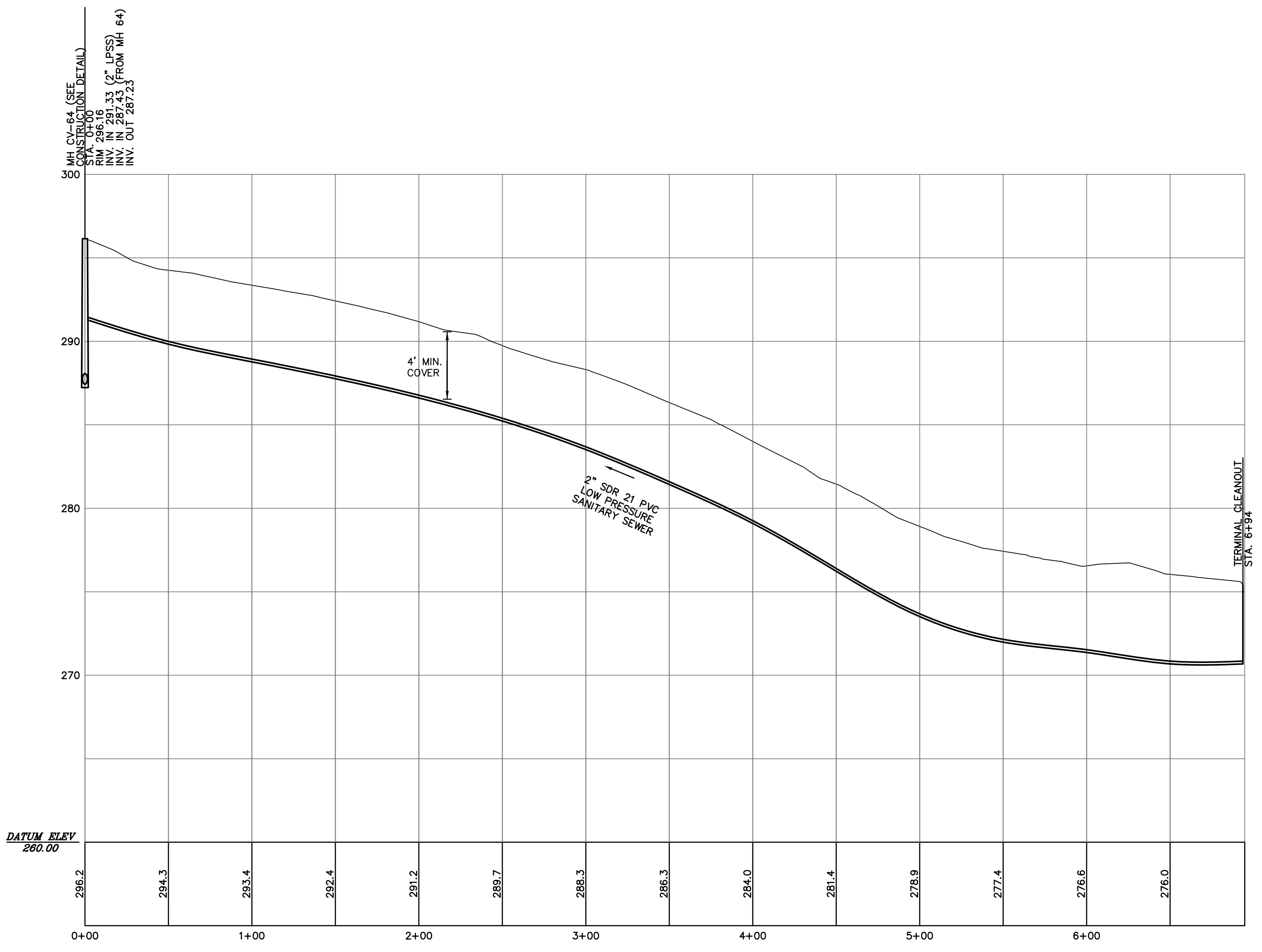
PROFILE: DOE RUN ROAD (STA. 0+00 TO 6+94) SCALE: HORIZ. 1"=50' VERT. 1"=5'
